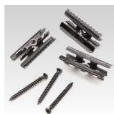
2.5 m² pack 50 Electrophoretic Coated Grab Deck Clips with 40 mm Torx Head wood screws and T15 bit
